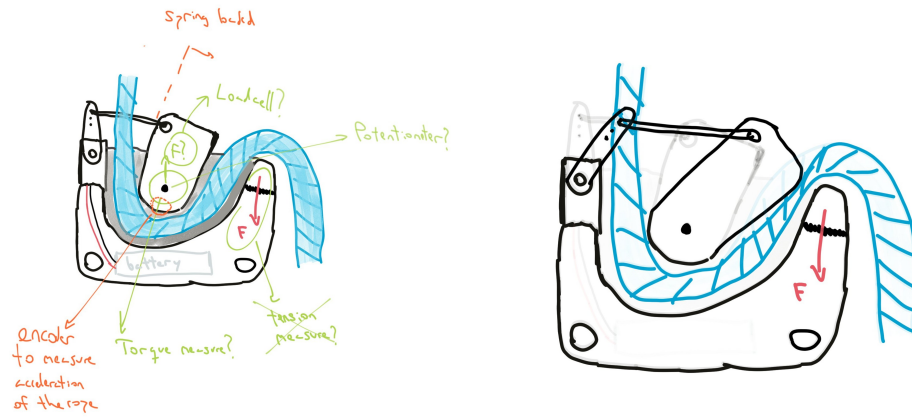
(a) Device with the required functions marked. (b) Device when the pinching mechanism is actuating.
